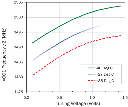
VCO1 Frequency versus Tuning Voltage For the same coarse tune setting, LO divide by two
