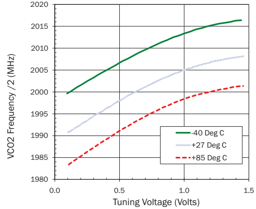
VCO2 Frequency versus Tuning Voltage For the same coarse tune setting, LO divide by two
