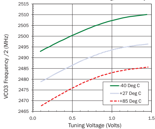
VCO3 Frequency versus Tuning Voltage For the same coarse tune setting, LO divide by two
