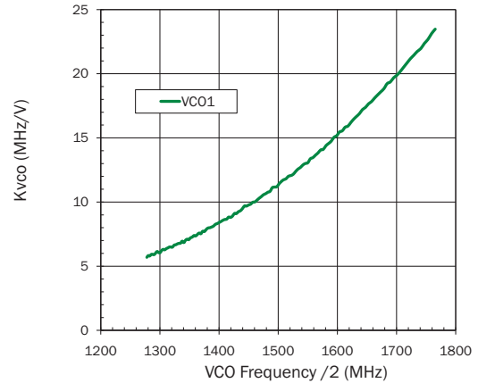
VC01 Frequency versus Kvco LO Divide by 2
