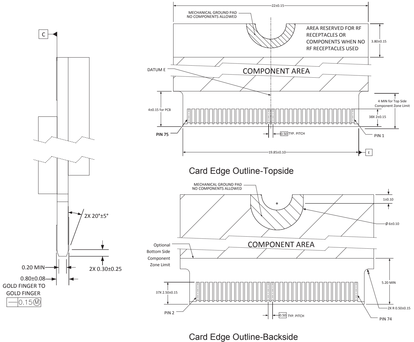
Figure 5: Dimensions Detail
