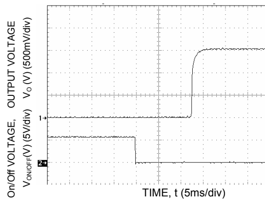
Figure 36. Typical Start-Up Using Remote On/Off, negative logic version shown.
