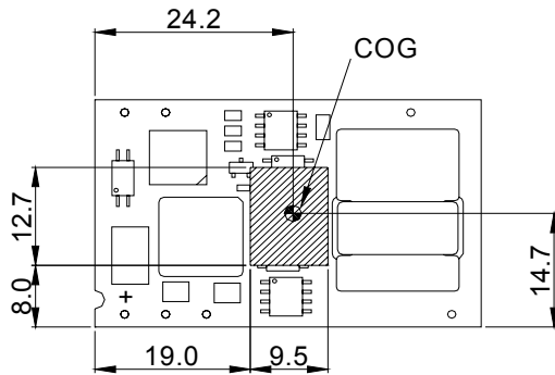
Note: All dimensions in mm. Figure 70. Pick and Place Location.
