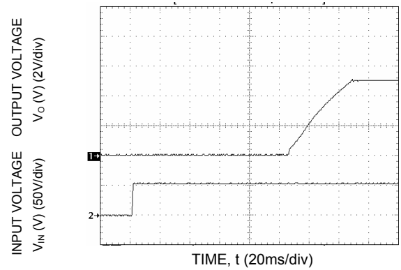
Figure 5. Typical Start-Up with application of Vin.
