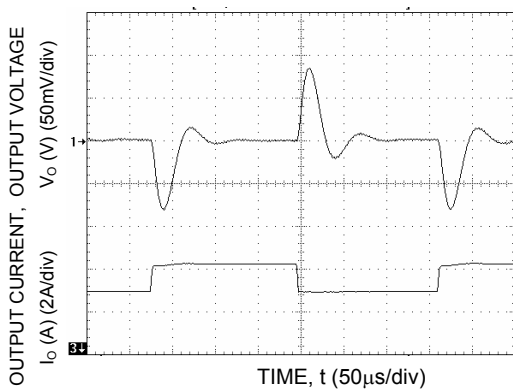
Figure 33. Transient Response to Dynamic Load Change from 50% to 75% to 50% of full load.
