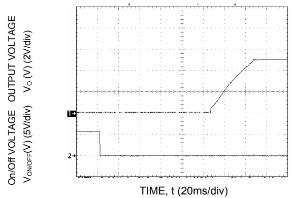
Figure 6. Typical Start-Up Using Remote On/Off, negative logic version shown.
