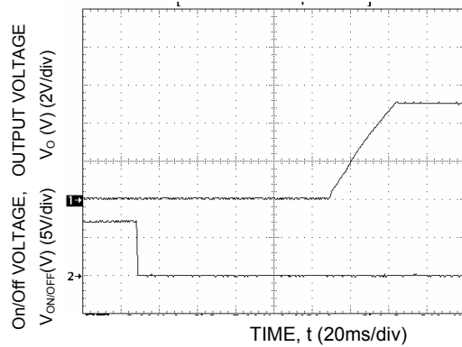
Figure 54. Typical Start-Up Using Remote On/Off, negative logic version shown.
