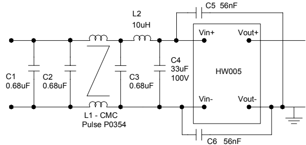
Figure 67. Suggested Configuration for EN55022 Class B.
