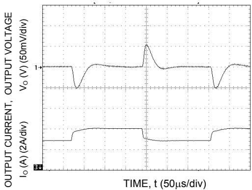
Figure 45. Transient Response to Dynamic Load Change from 50% to 75% to 50% of full load.
