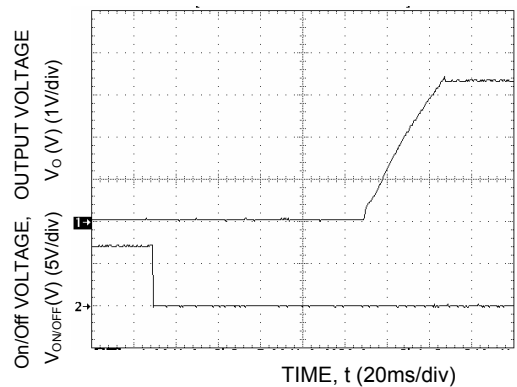
Figure 60. Typical Start-Up Using Remote On/Off, negative logic version shown.
