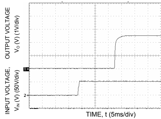
Figure 17. Typical Start-Up with application of Vin.
