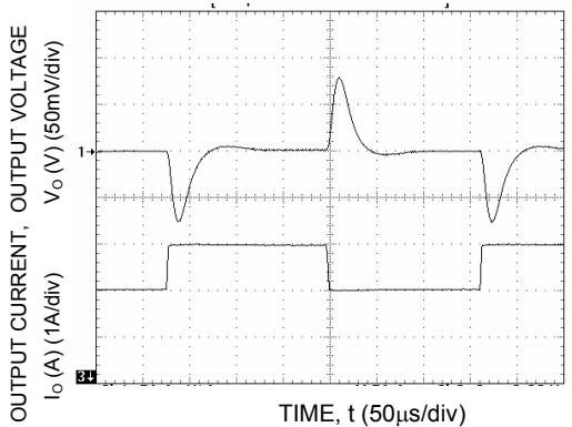
Figure 51. Transient Response to Dynamic Load Change from 50% to 75% to 50% of full load.
