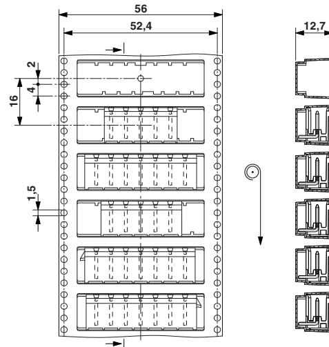
Dimensioned drawing
