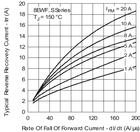
Fig. 13 - Recovery Current Characteristics, T_J = 150\text{ }^\circ\text{C}
