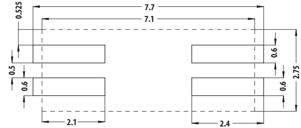
Figure 10. Land Pattern
