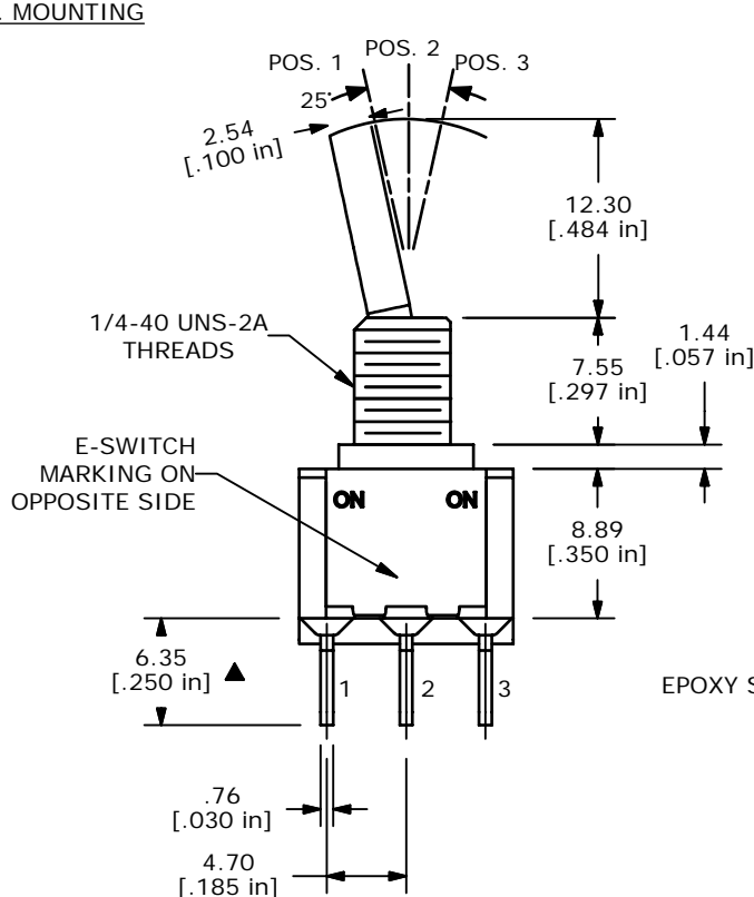
P.C.B. MOUNTING
