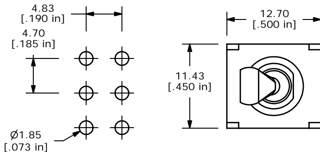
P.C.B. MOUNTING
