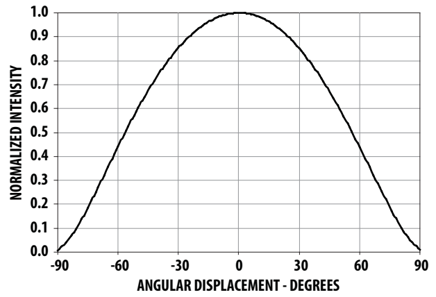
Figure 9. Radiation Pattern
