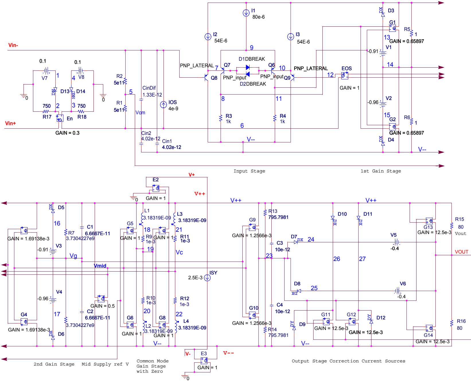
FIGURE 64. SPICE SCHEMATIC
