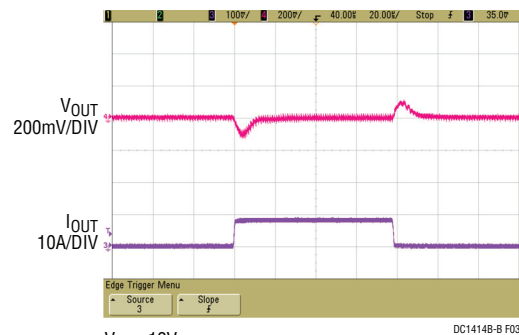
V_{IN} = 12V V_{OUT} = 1.2V 2A TO 10A LOAD STEP C_{OUT} = 2 \times 100\mu F, 3.6V, X5R, 1812 CERAMIC + 1 \times 22\mu F, 10V, X5R, 1206 CERAMIC
