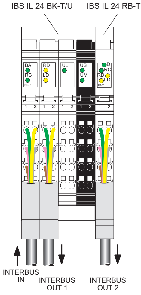
Figure 4 Example of connecting the INTERBUS cables to the bus terminal and to the remote bus branch terminal
