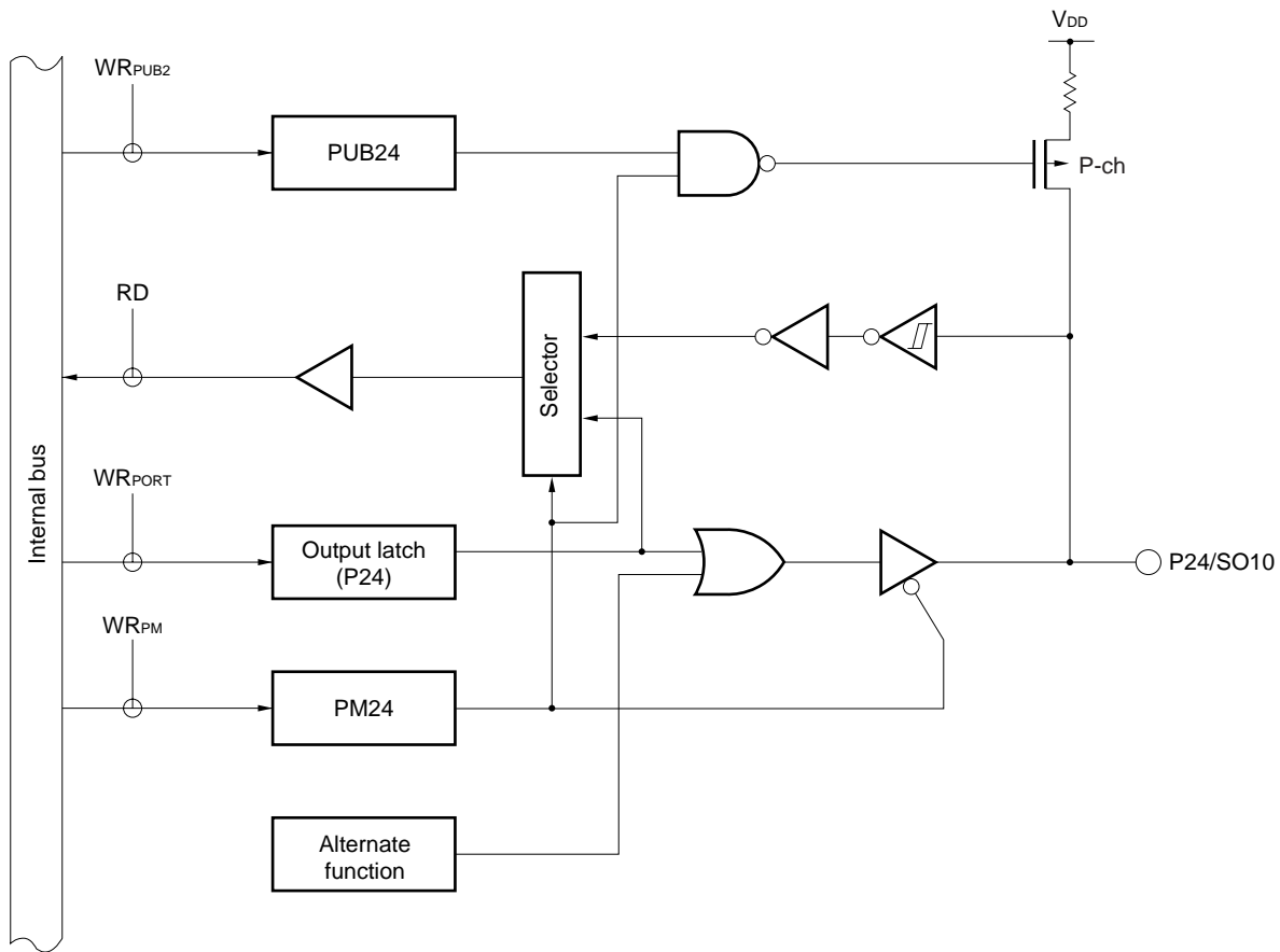
Figure 4-8. Block Diagram of P24
