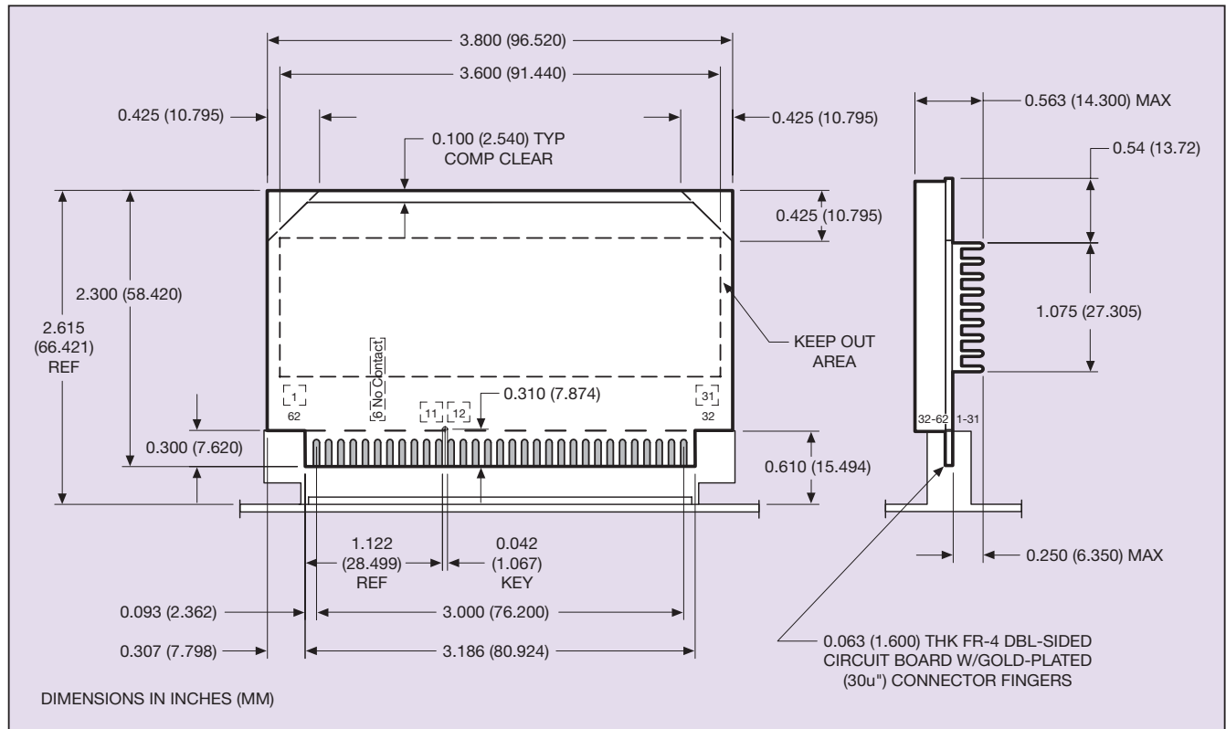
Figure 1: Mechanical Drawing
