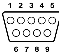
Figure 2.18 LCD Backlight connector
