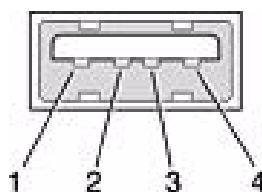
Figure 2.10 USB connector
