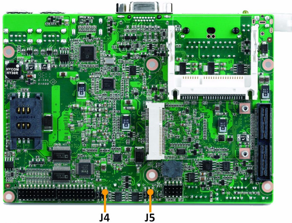
Figure 2.2 Jumper layout (Solder Side)
