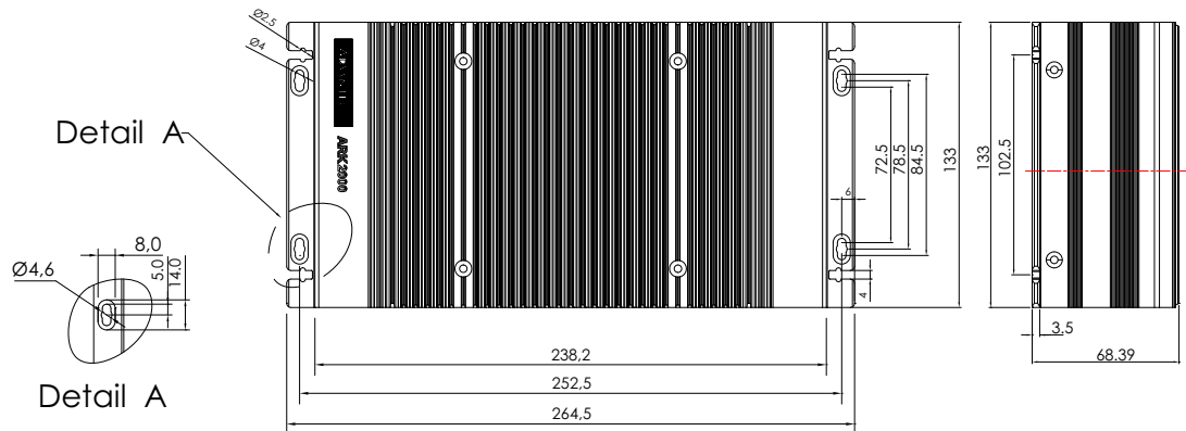
Figure 1.1 ARK-2120 Mechanical dimension drawing
