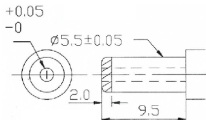
Figure 2.13 Compatible dimension of DC Plug for ARK-2120L
