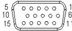
Figure 2.11 VGA Connector
