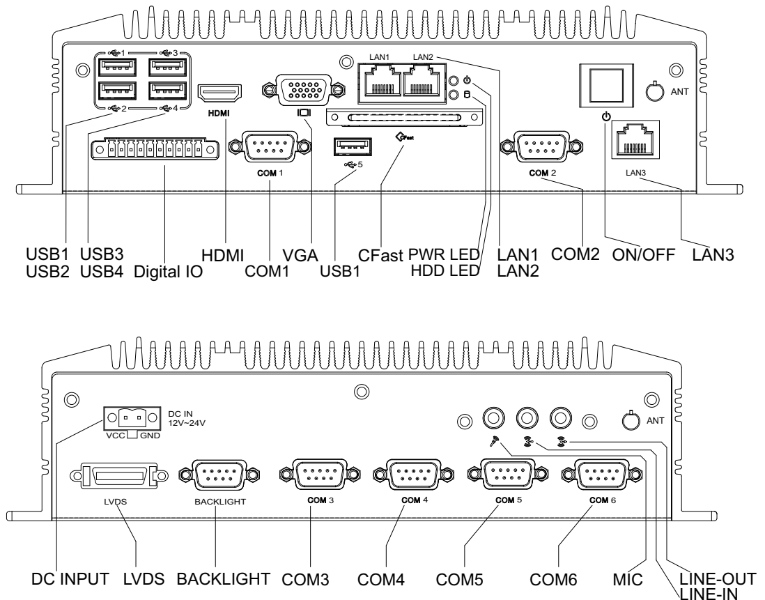
Figure 2.4 ARK-2120F IO connectors drawing
