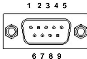
Figure 2.5 COM connector
