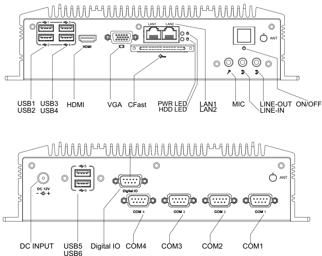
Figure 2.3 ARK-2120L IO connectors drawing
