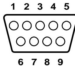
Figure 2.8 DIO Connector (ARK-2120L)
