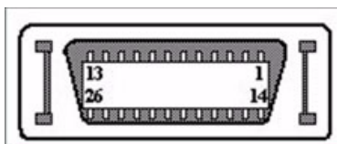
Figure 2.17 LVDS Connector
