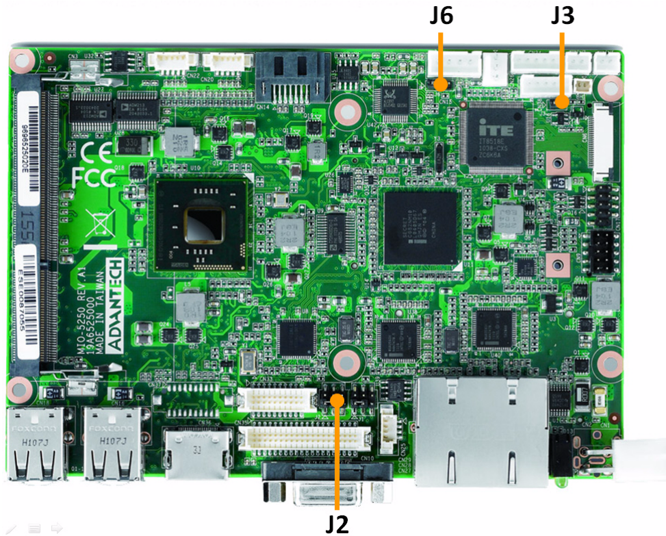
Figure 2.1 Jumper layout (Component Side)
