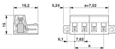
Dimensioned drawing
