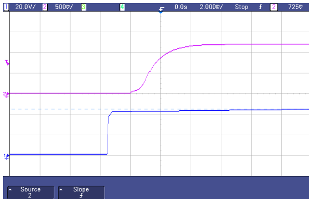
Fig.21 Typical start-up from power on of AGQ100-48S1V2
