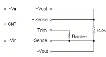
Fig. 54 Trim down circuit
