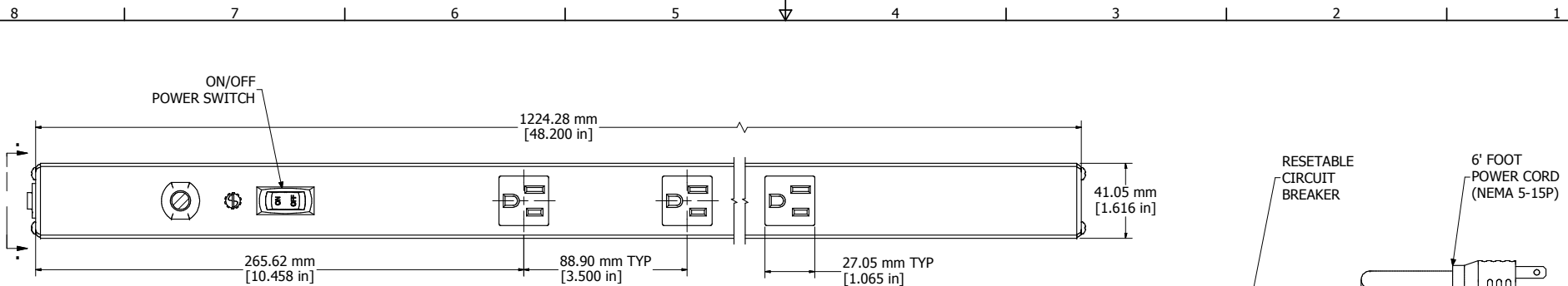
SECTION A-A (VIEW FROM FRONT)
