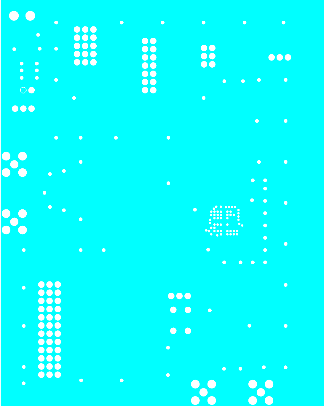
Figure 6. Si5320-EVB—Layer 4, VDD 2.5
