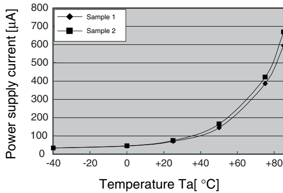
Power supply current (stop mode)
