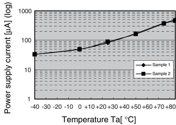
I_{CCCT} temperature characteristics (semi-log) V_{CC} = 3.3\text{ V}
