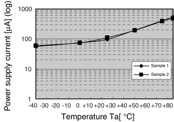
I_{CCCL} temperature characteristics (semi-log) V_{CC} = 3.3\text{ V}
