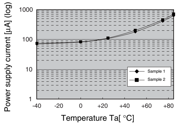
I_{CC1} temperature characteristics (semi-log) V_{CC} = 3.3\text{ V}
