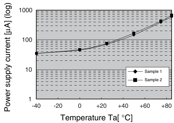
I_{CC2} temperature characteristics (semi-log) V_{CC} = 3.3\text{ V}
