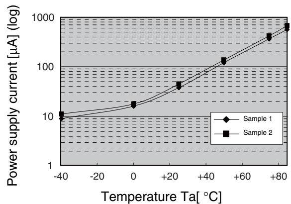
I_{CC3} temperature characteristics (semi-log) V_{CC} = 3.3\text{ V}
