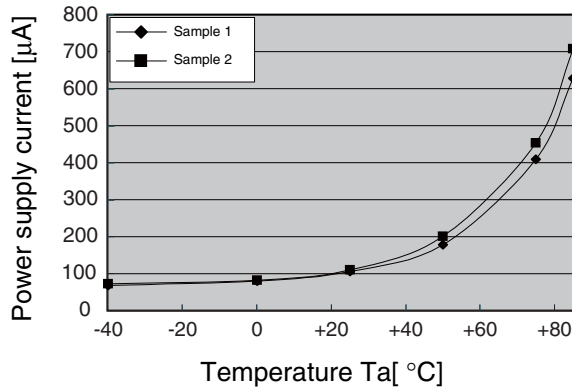
Power supply current (watch mode)
