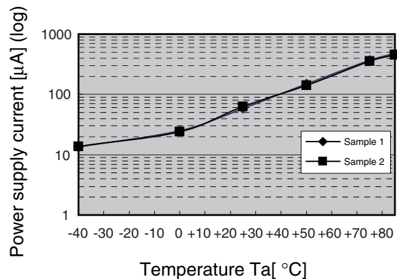
I_{CCH} temperature characteristics (semi-log) V_{CC} = 3.3\text{ V}
