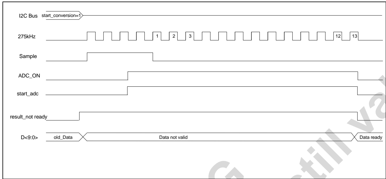
Figure 24. ADC Timing-diagram
