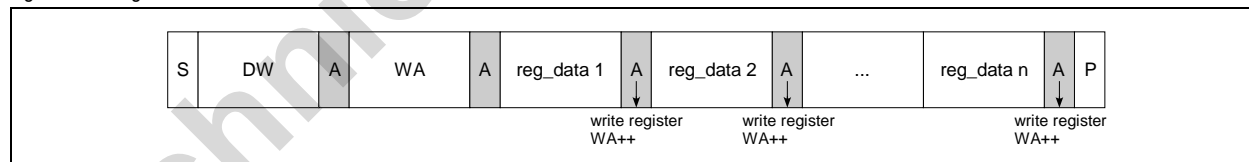
Figure 26. Page Write
