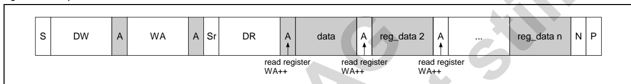
Figure 28. Sequential Read
