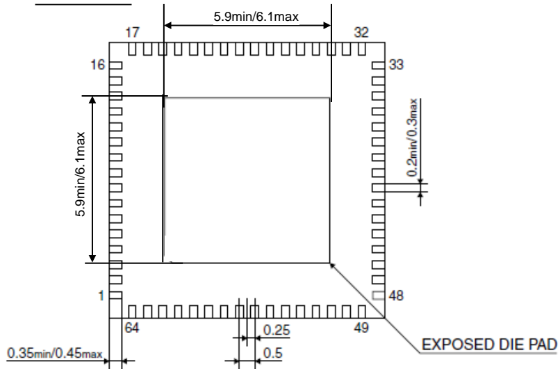
Figure 25.1 SQFN9-64pin Package Dimensions
