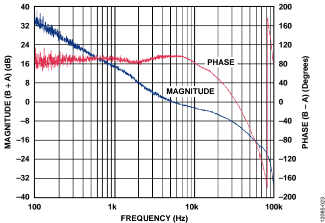
Figure 23. Control Loop Test Using an AP300 Loop Analyzer
