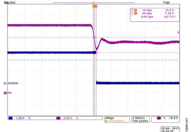
Figure 40. A VOUT_UV_FAULT Flag to Trigger PGOOD Output
