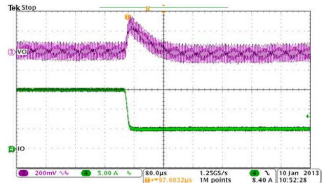
Figure 25. Transient Response with Load Steps: 50% to 75% to 50%
