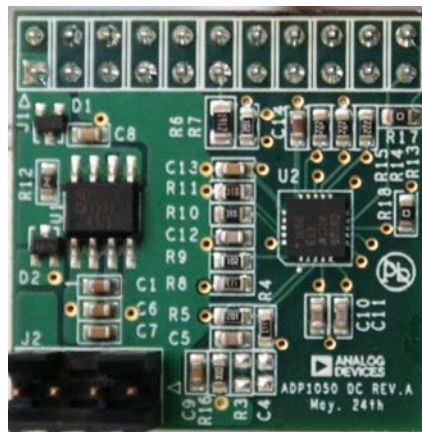
Figure 3. ADP1050DC1-EVALZ Daughter Card
