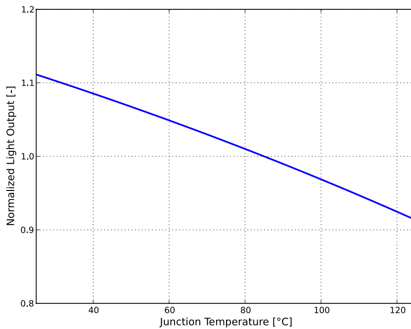
Figure 2. Typical normalized light output vs. junction temperature for LUXEON CoB with FreshFocus Technology at specified test current.
