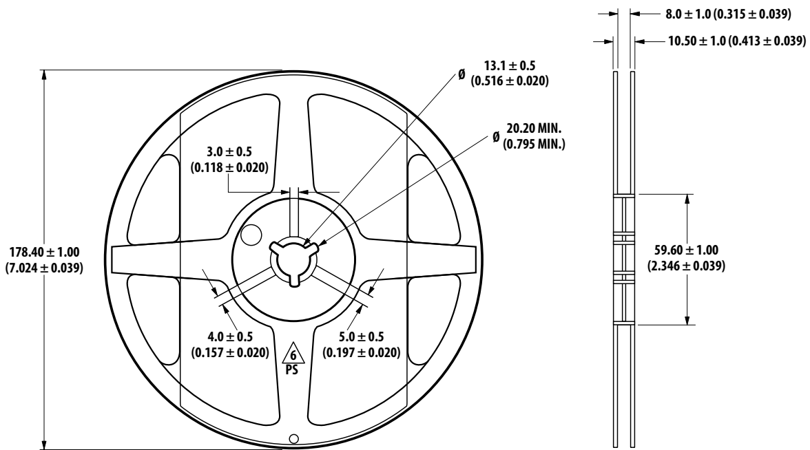
Figure 15. Reel Dimension
