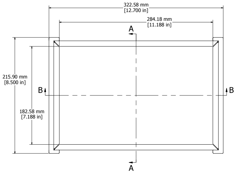
Assembly - View From Bottom
